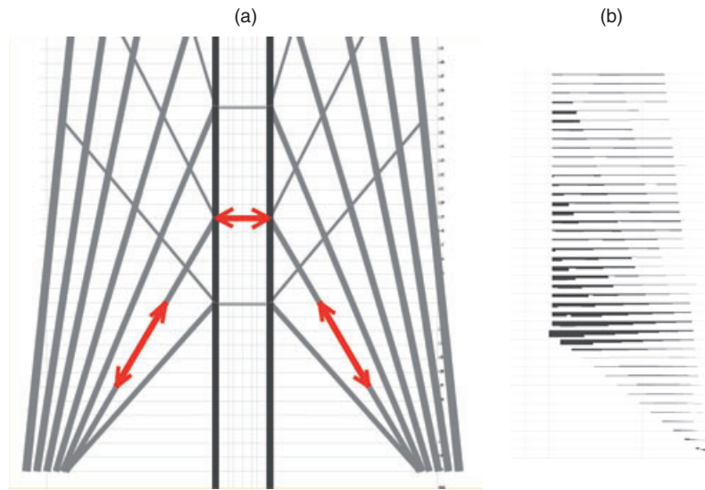
Figure 8. Gravity load path diagrams: (a) in fan column and links; (b) in spandrel beams
