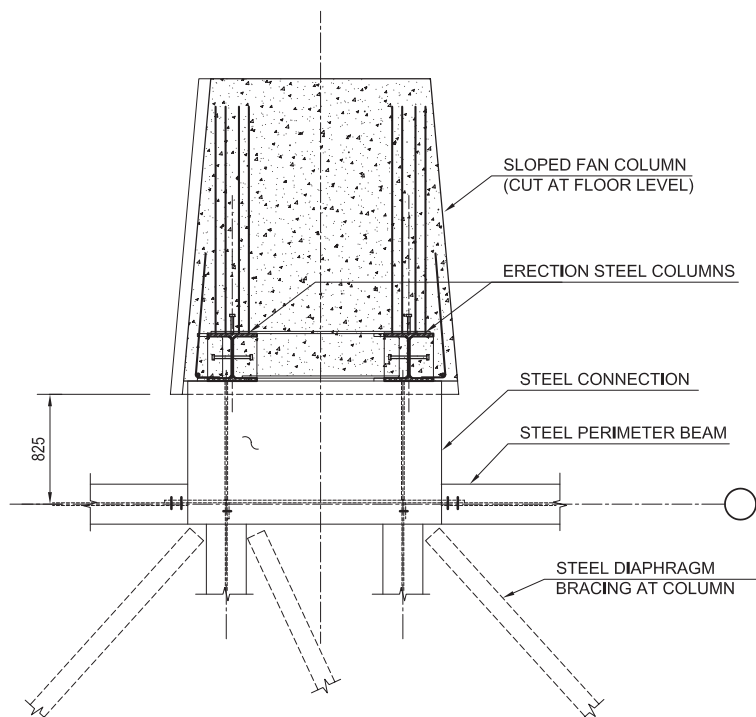
Figure 10. Connection of fan column to floor framing
