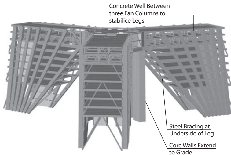
Figure 13. Base of tower structure
