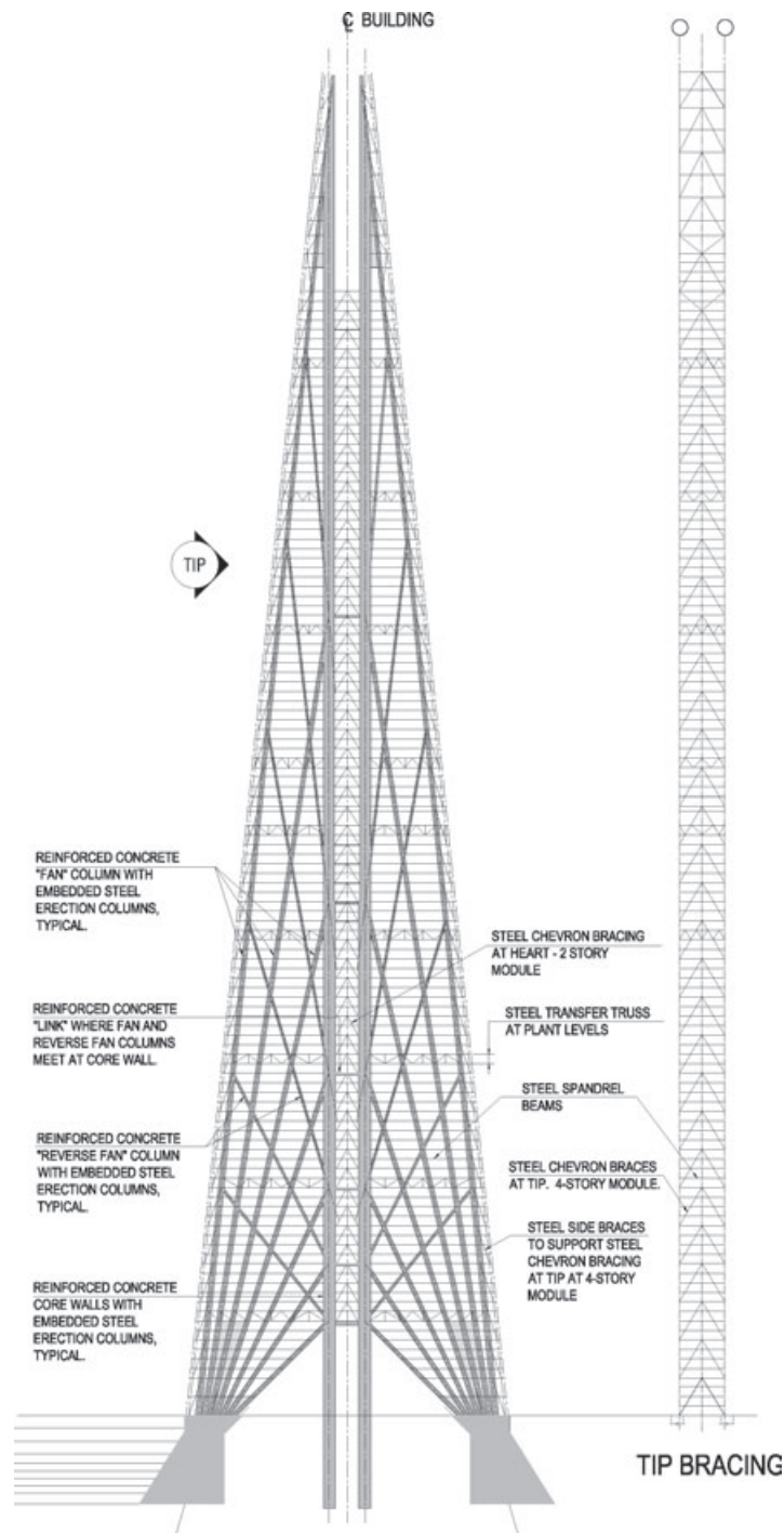
Figure 11. Structural system summary elevation
