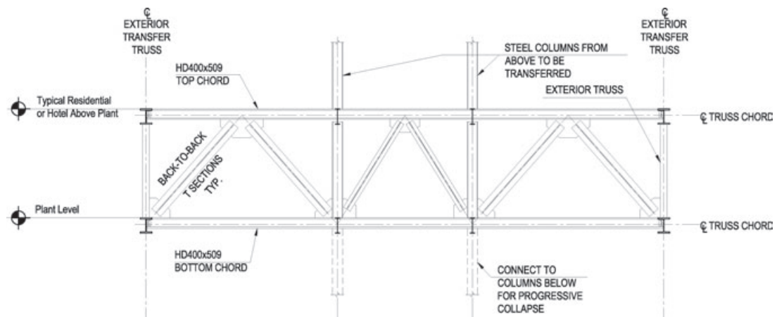
Figure 15. Full-depth transfer truss at plant levels
