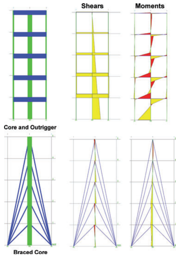
Figure 7. Lateral load path diagrams
