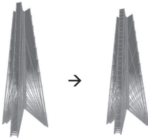
Figure 9. Solving torsion issue—add reverse fan columns on façade
