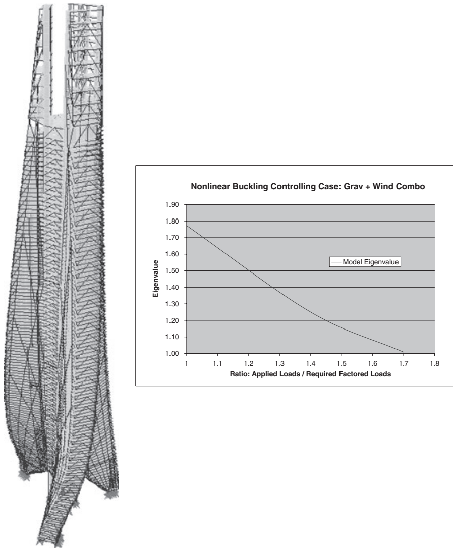
Figure 16. Torsional buckling of tower at ratio of 1.7 \times factored loads (including wind) or 2.1 \times service loads
