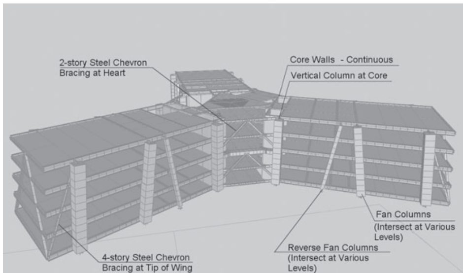
Figure 17. Four-story portion of tower showing varied modules of bracing
