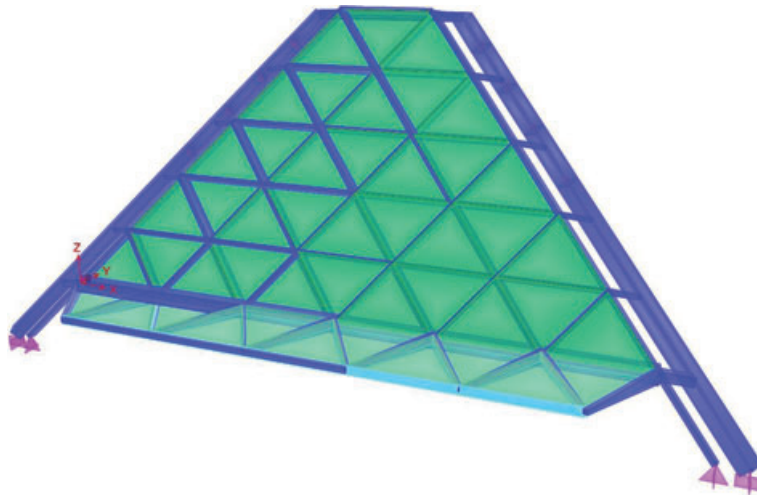
Figure 14. Structural model of atrium structural steel and glass roof enclosure
