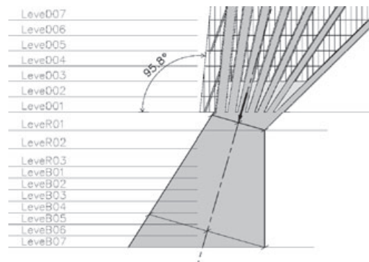
Figure 12. Fan column abutment
