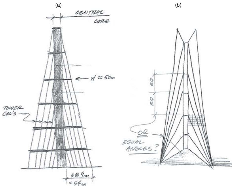
Figure 6. Reaching current structural form. (a) Parallel sloped columns. (b) Sloped columns to one point
