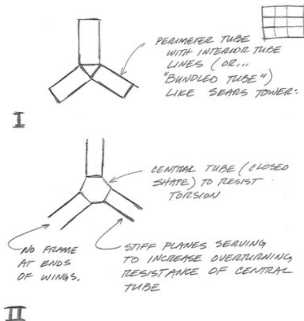
Figure 4. Early structural plan concepts
