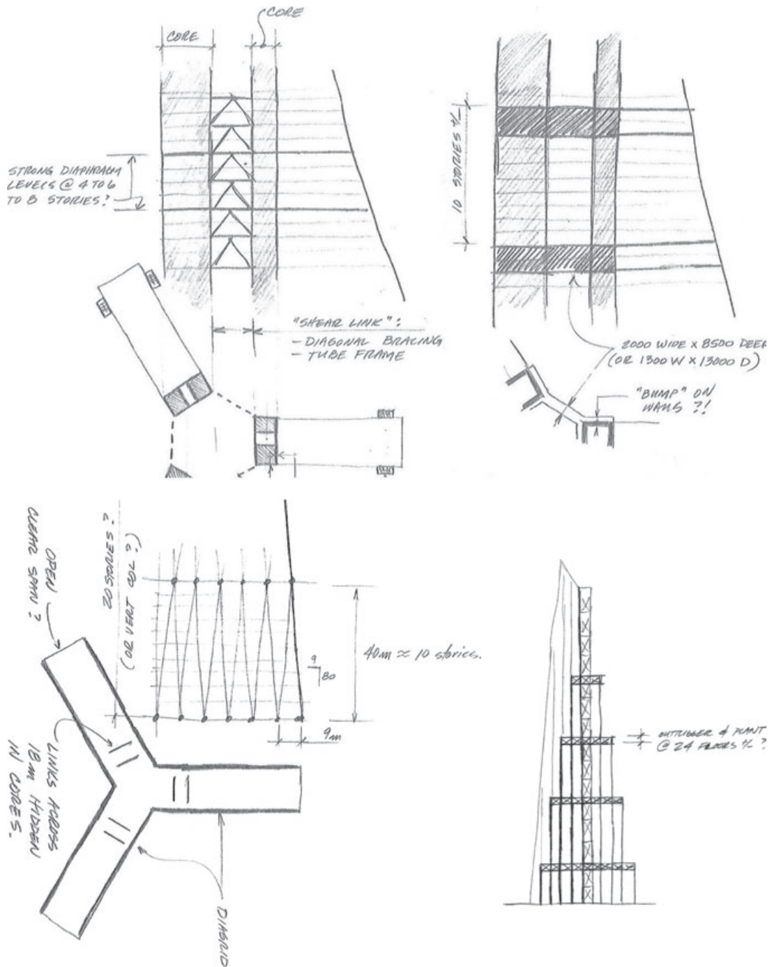
Figure 5. Early structural system concept sketches
