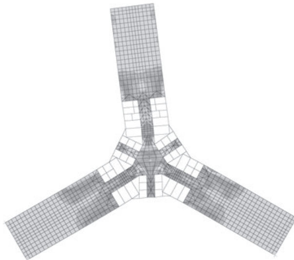
Figure 18. Diaphragm stresses due to horizontal loads
