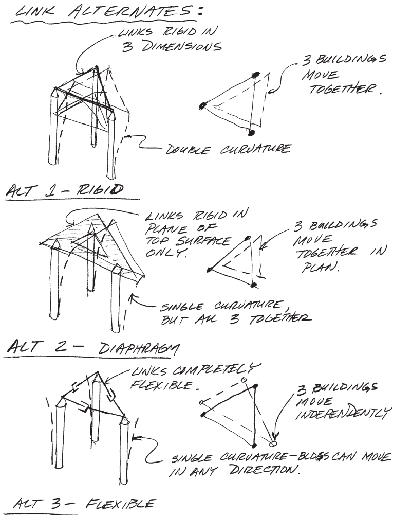
Figure 2. Structural concepts for linking towers
